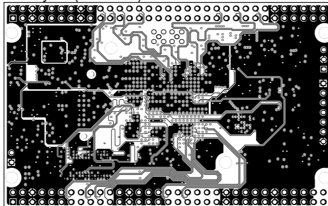
MidLayer2 (Scale 1:1)
