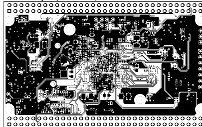
BottomLayer (Scale 1:1)
