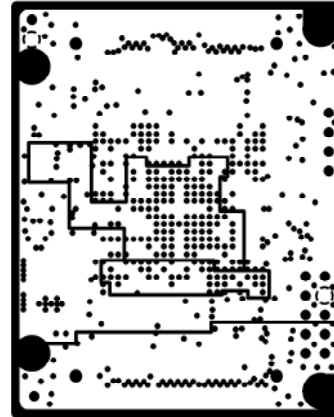
INTERNAL PLANE3
