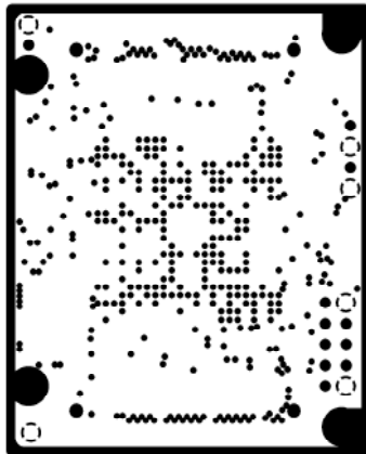
INTERNAL PLANE1(GND)
