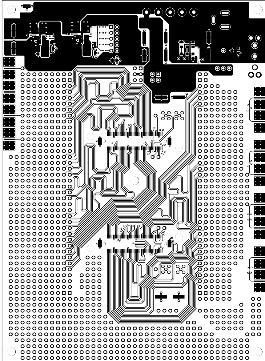
TopLayer (Scale 1:1)
