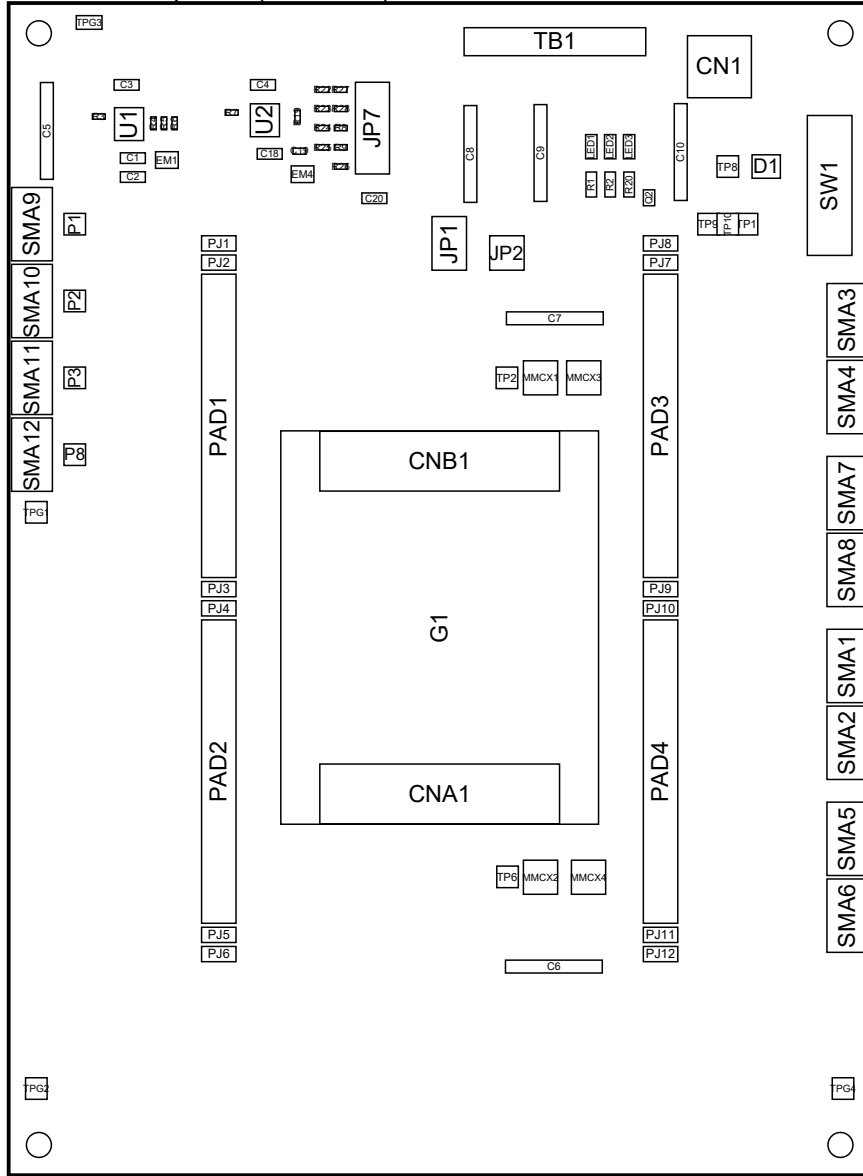
View from Top side (Scale 1:1)
