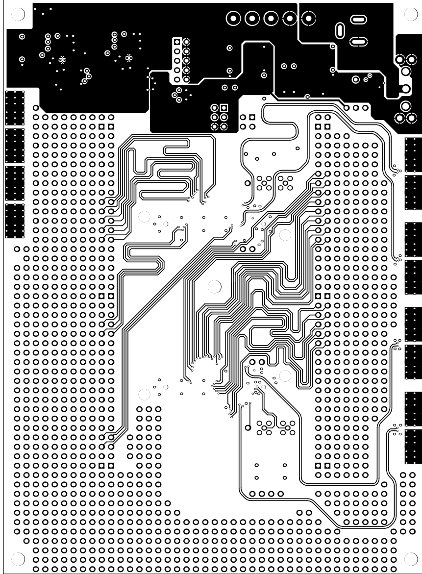
BottomLayer (Scale 1:1)
