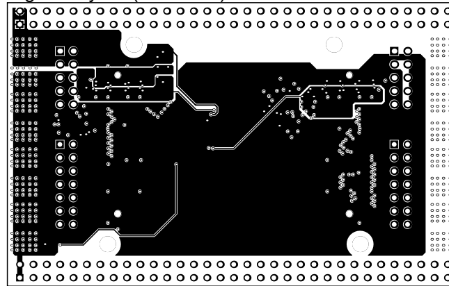
BottomLayer (Scale 1:1)
