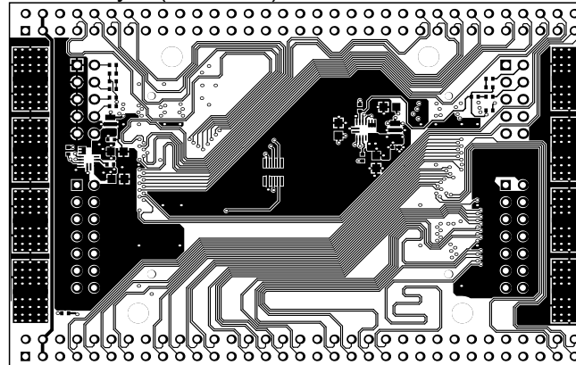
BottomLayer (Scale 1:1)
