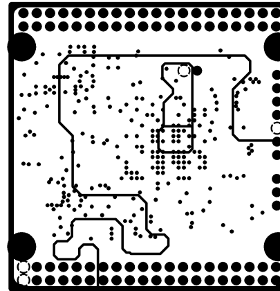
INTERNAL PLANE2
