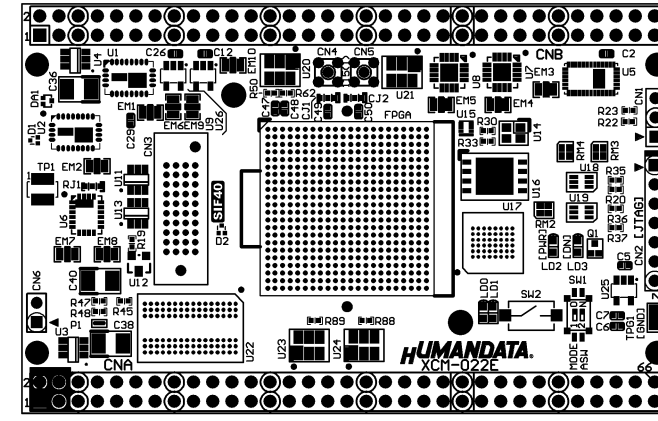
Component Side
