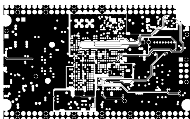
MID LAYER4
