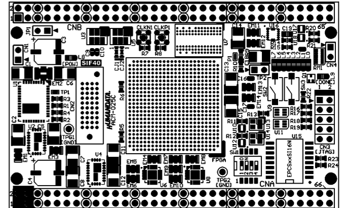
Component Side
