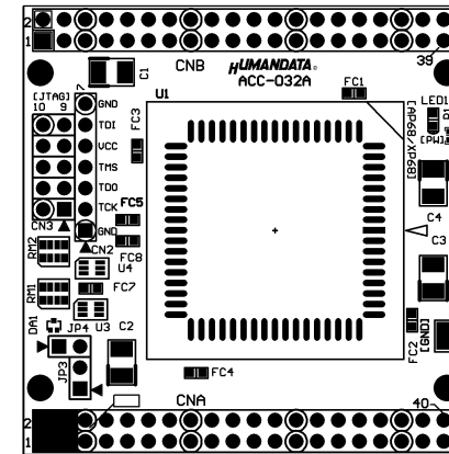
Component Side
